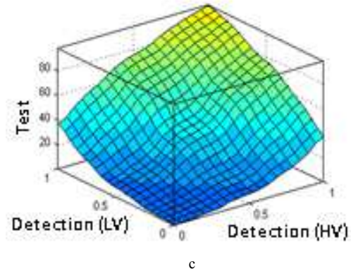
Fig. 7. a – Dependence of expediency of inclusion j^{th} of the test in the program of tests from probability of display of i^{th} malfunction, which it covers with low value of probability of malfunction's display; b – Dependence of expediency of inclusion j^{th} of the test in the program of tests from probability of display of i^{th} malfunction, which it covers with high value of probability of malfunction's display; c – Dependence of expediency of inclusion of the test in the program of tests from probability of display of i^{th} malfunction and probability of its covering by the given test.
