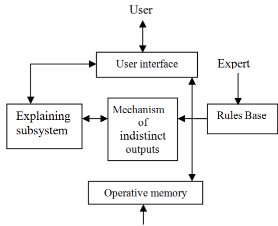
Fig. 6. Structure of expert system.
