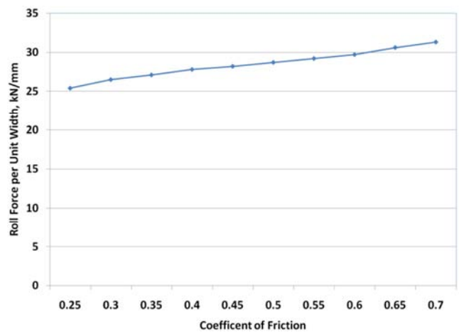
Figure 6. Average pass roll force at different coefficient of friction with 30% reduction.
