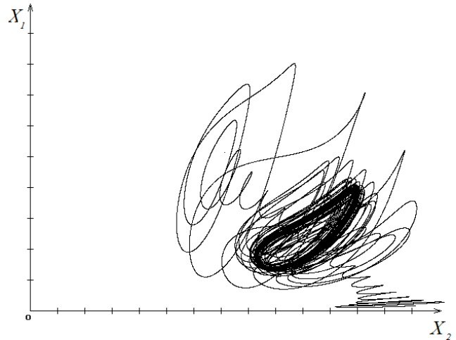
Figure 7. Chaos in the model system for equation (2).
