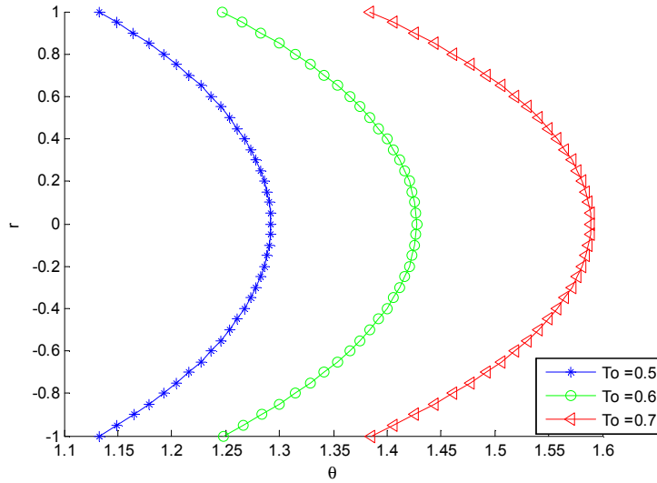
Figure 31. Effect of varying parameter T_o on the temperature distribution of Vogel's viscosity model under slip condition when for A = -C = \delta = \gamma = 1 .
