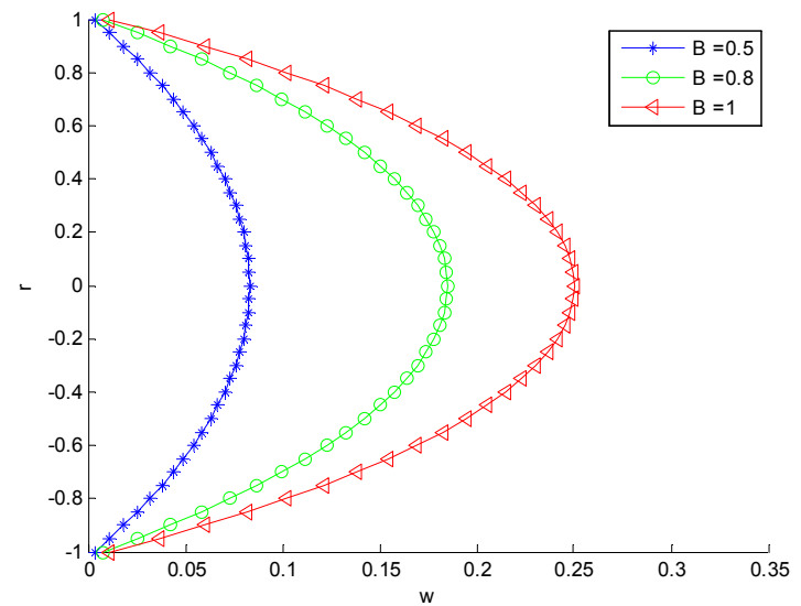
Figure 7. Effect of varying parameter B on the velocity distribution of Reynolds viscosity model when for A = \delta = C = \gamma = \Gamma = 1 .
