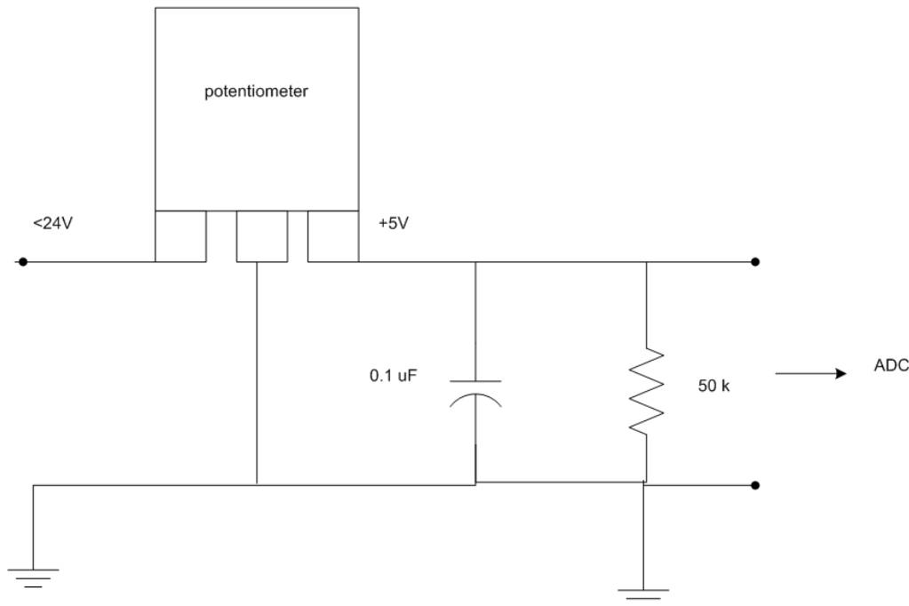
Figure 4. Potentiometer.
